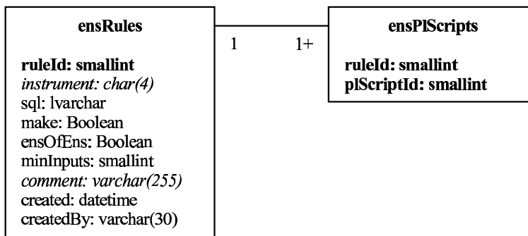
Figure 2. Schema for the ensRules and ensPIScripts database tables.
