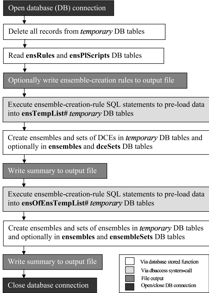
Figure 3. Flow chart for the perl script createEnsembles.pl.
