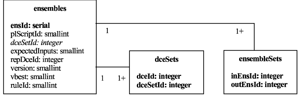
Figure 1. Schema for the ensembles, dceSets, and ensembleSets database tables.
