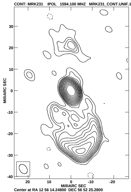
Figure 2. 18 cm VLBI image of the central 100pc of Mrk 231, interpreted as a nascent QSO; age < 10^6 yr.
